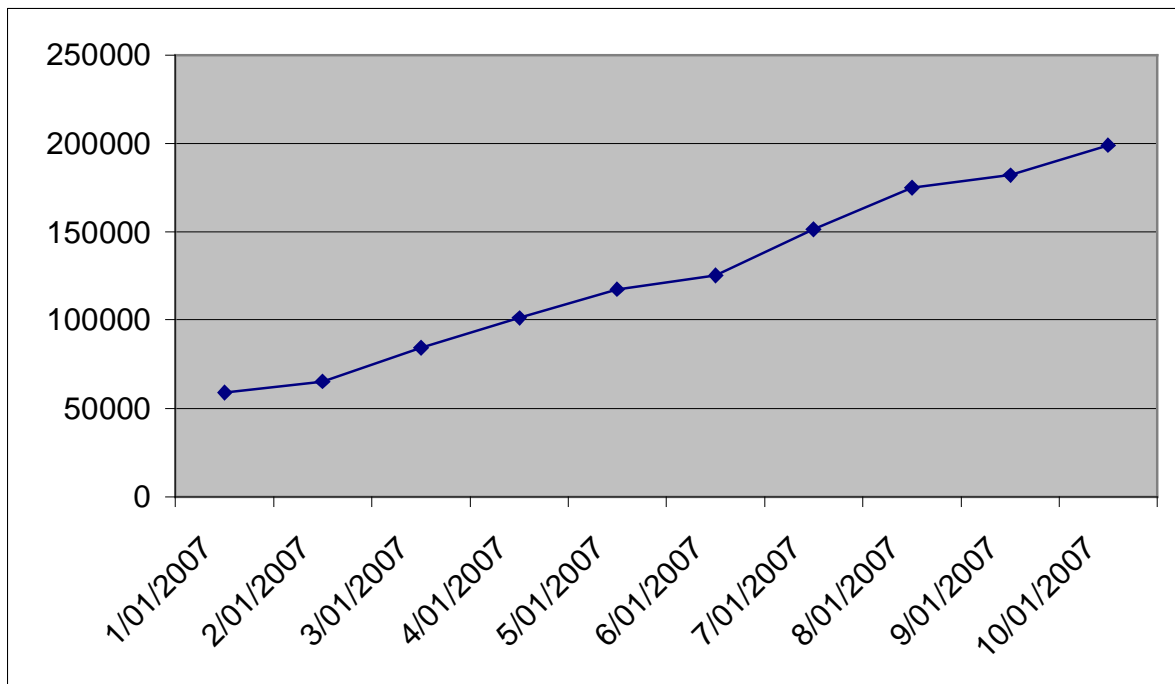
Equity curve Blue Monthly return
